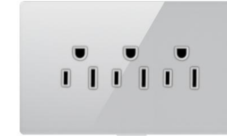
U2.1-036 3 Gang American socket 15A 125V 16A 250V
