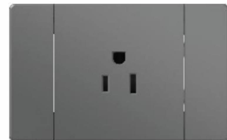
U110-015 1 Gang American socket 15A 125V 16A 250V
