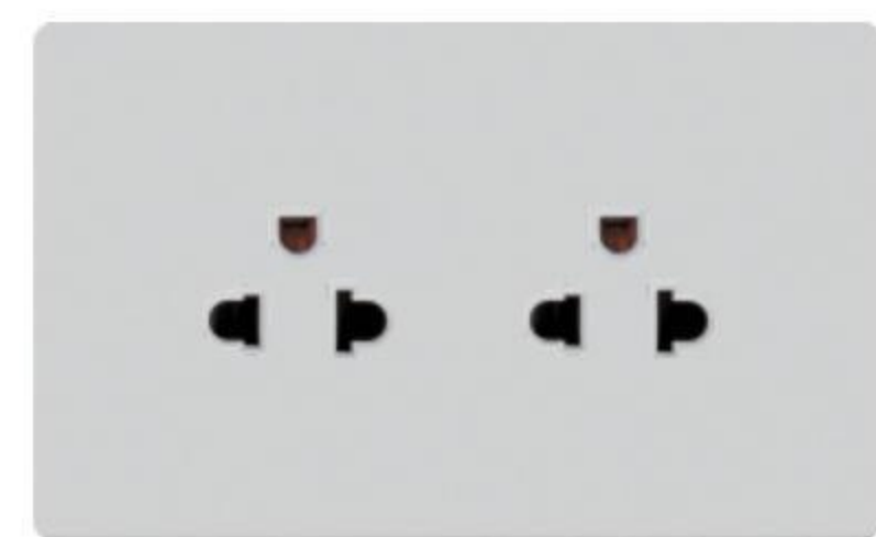
U1.1-010 2 Gang American multi socket 15A 125V 16A 250V
