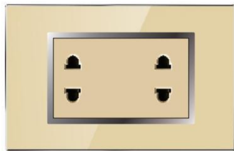
N8-037 2 Gang American socket 15A 125V 16A 250V
