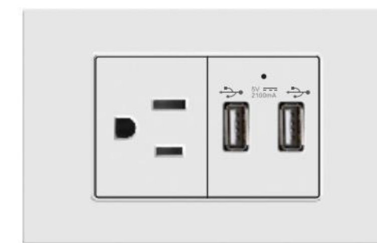
N1.9-018 1 Gang American multi socket and 2 USB 15A 125V 16A 250V
