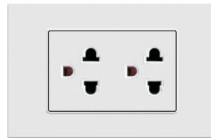
N1.9-010 2 Gang American multi socket 15A 125V 16A 250V
