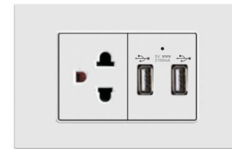
N1.9-013 1 Gang American multi socket and 2 USB 15A 125V 16A 250V
