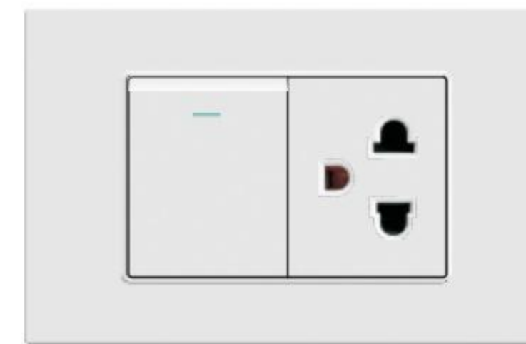
N1.9-011 1 Gang 1 way switch and American multi socket N1.9-012 1 Gang 2 way switch and American multi socket
