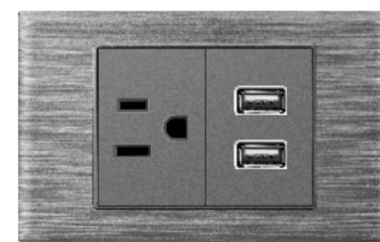
H200-018 1 Gang American multi socket and 2 USB 15A 125V 16A 250V
