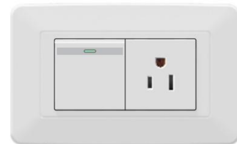
118Z-07 1Gang 1 way switch+Single socket 118Z-07(3 way) 1Gang 2 way switch+Single socket 10-16A 110-250V~
